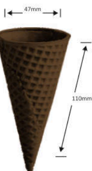
FLAVOURED Sugar Rolled Cones-110mm Height: 110mm \pm 3mm Weight: 11gm \pm 1gm Angle-23° Product Code FCB-110
