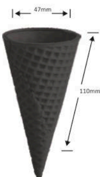
FLAVOURED Sugar Rolled Cones-110mm Height: 110mm \pm 3mm Weight: 11gm \pm 1gm Angle-23° Product Code FCB-110
