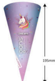
Cone Sleeves-195mm Height: 195mm \pm 2mm Angle-22° Product Code CS-195
